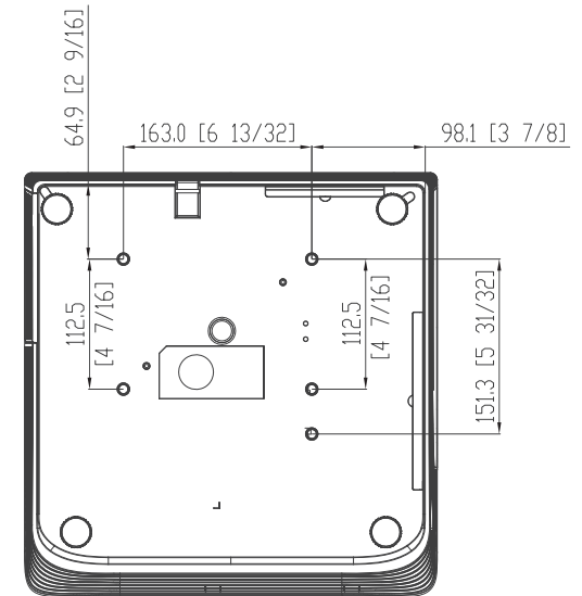
Mounting Surface
