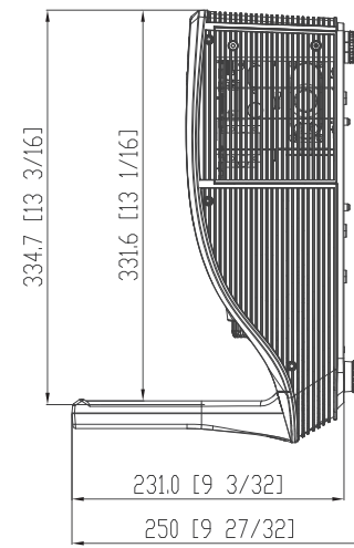
Lamp Side
